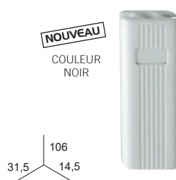
CONTREPOIDS 70 gr.
