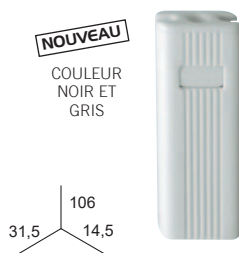
CONTREPOIDS 110 gr.
