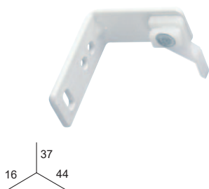
SUPPORT 3 cm.
