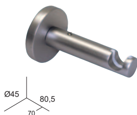
SUPPORT SIMPLE
