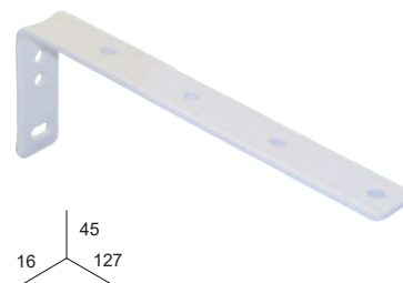
SUPPORT MUR 12 cm. (Pour ref. 7286400)
