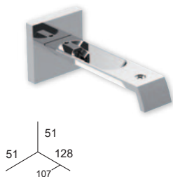
SUPPORT
