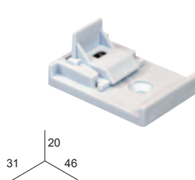
SUPPORT PLAFOND
