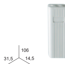
CONTREPOIDS 70 gr.
