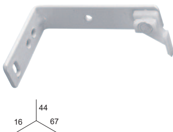
SUPPORT 6 cm.
