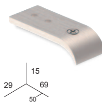
SUPPORT PLAFOND
