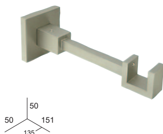
SUPPORT
