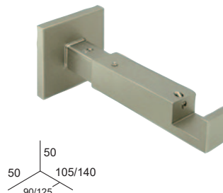
SUPPORT EXTENSIBLE
