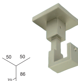
SUPPORT PLAFOND
