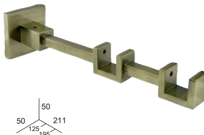
SUPPORT DOUBLE
