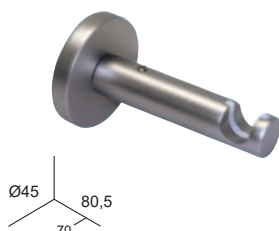
SUPPORT SIMPLE
