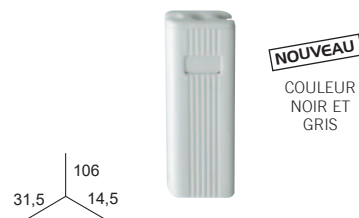
CONTREPOIDS 70 gr.
