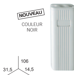
CONTREPOIDS 70 gr.
