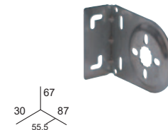
SUPPORT MECANISME Ø47
